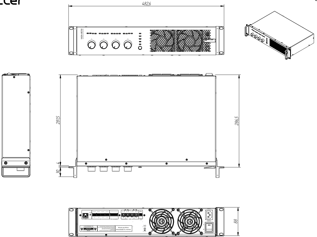
Ecler HADA-4B750 Mechanical Diagram
