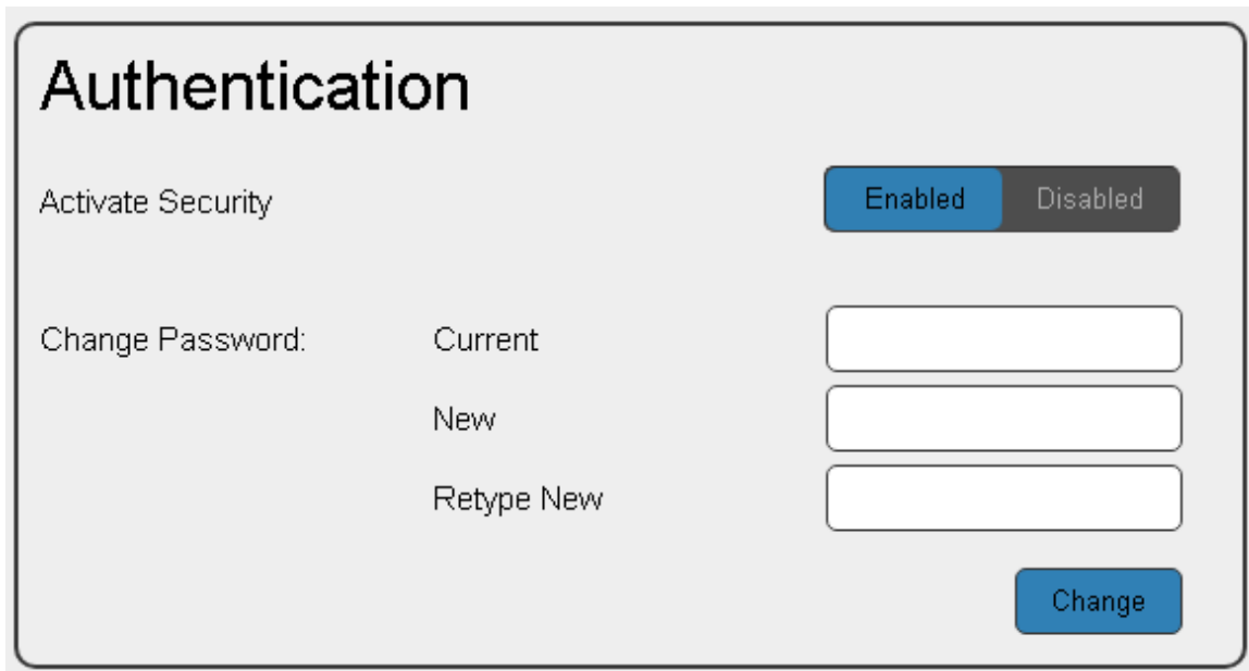
Figure 23: Authentication Page
