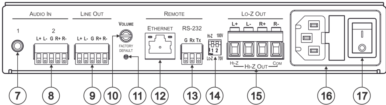
Figure 3: PA-240Z and PA-120Z Rear Panel
