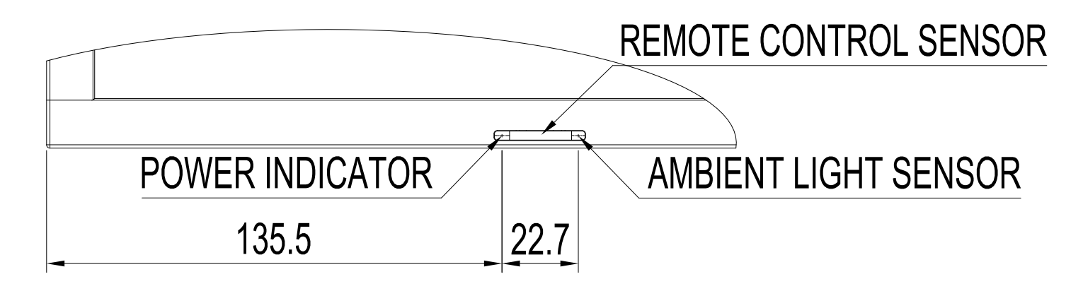
DETAIL C SCALE 3:1
