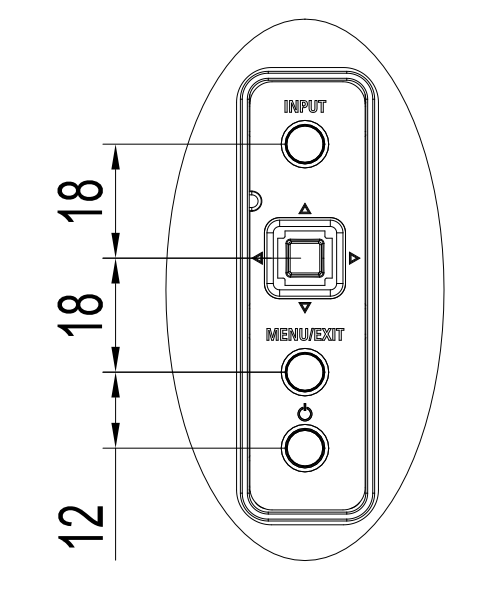
DETAIL E SCALE 4:1
