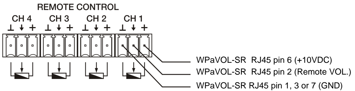
Connection of WPaVOL-SR to remote-control ports
