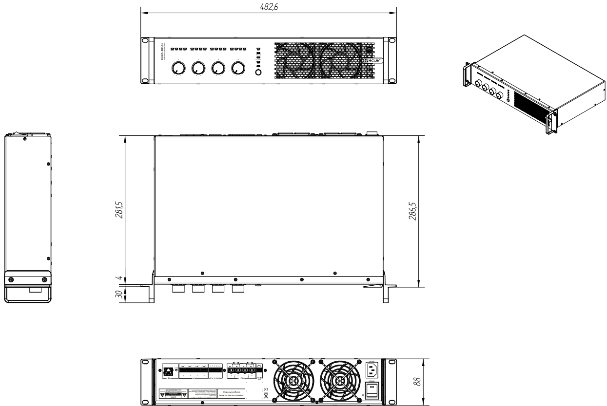
Ecler HADA-4B150 Mechanical Diagram
