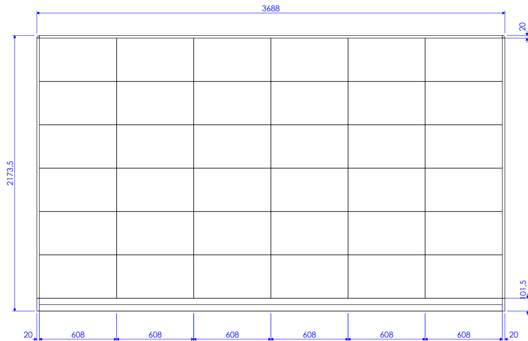
FRONT VIEW
